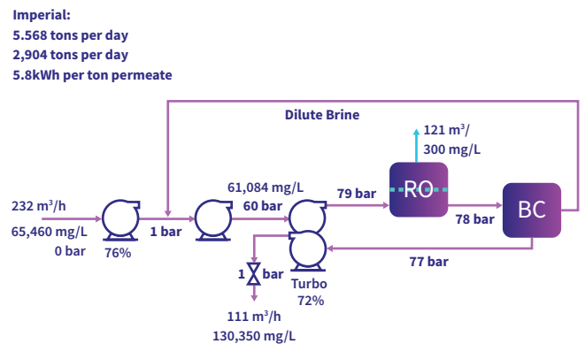
Figure 2. CFRO Process for Brine Desalination
